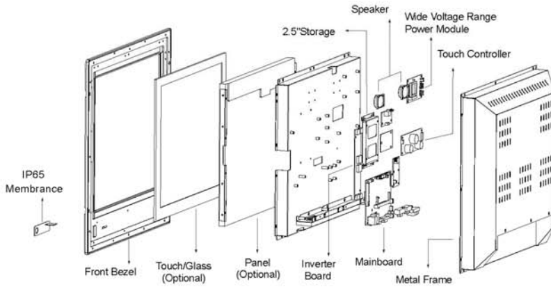
Modularized Construction
